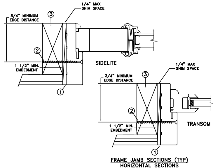
THROUGH FRAME INSTALLATION
